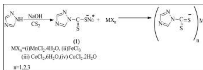
Fig 1 sequence of reactions
