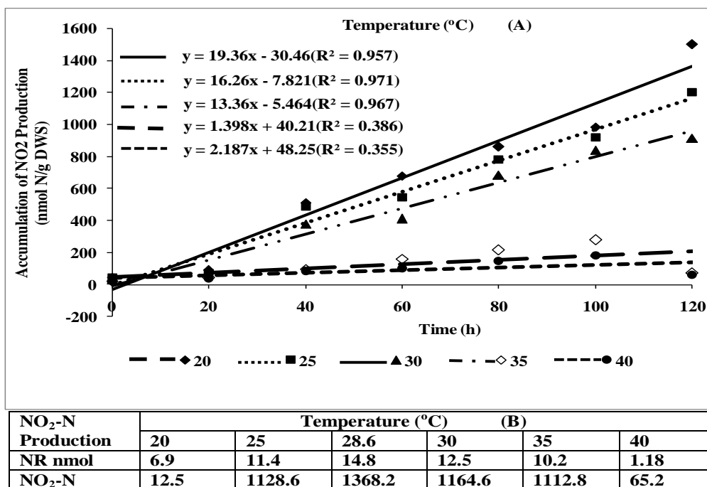
Figure 3: Nitrification rate (NR) of sediment at various temperatures determined by the accumulation of NO 2 production at 120h incubation (A). Relationship between temperature and NR (B).
