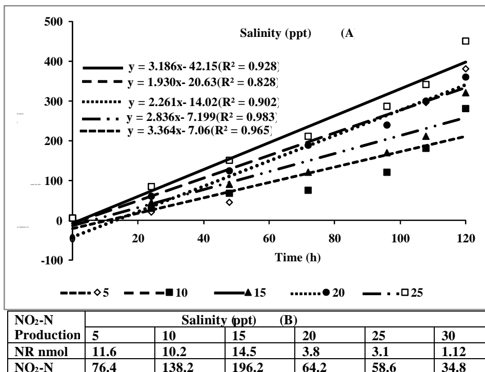
Figure 6 : Nitrification rate (NR) of sediment at various salinity determined by the accumulation of NC 2 production at 120h incubation (A) Relationship between salinies and NR (B).
