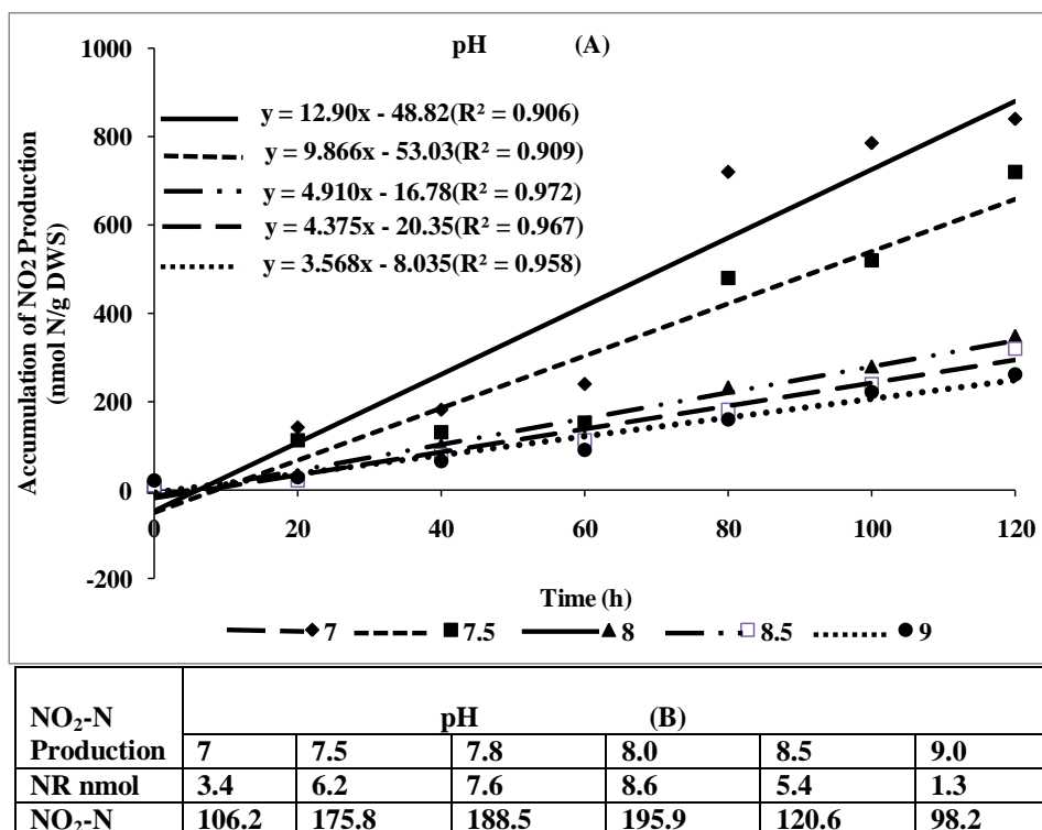
Figure 4: Nitrification rate (NR) of sediment at various pHs determined by the accumulation of NO 2 production at 120h incubation (A). Relationship between pH and NR (B).
