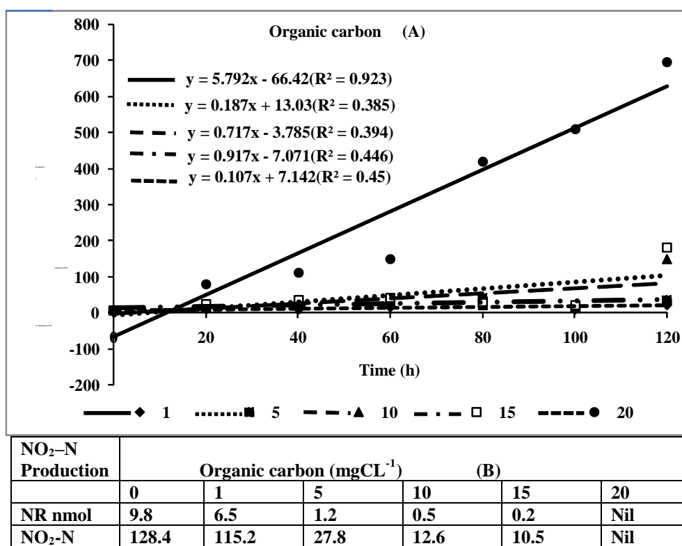
Figure 5: Nitrification rate (NR) of sediment at various organic carbons determined by the accumulation of NO 2 production at 120h incubation (A). Relationship between organic carbons and NR (B).
