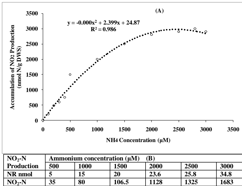
Figure 7: Nitrification rate (NR) of sediment at various concentration of \text{NH}_4\text{-N} determined by the accumulation of \text{NO}_2 production at 120h incubation (A). Relationship between \text{NH}_4\text{-N} and NR (B).
