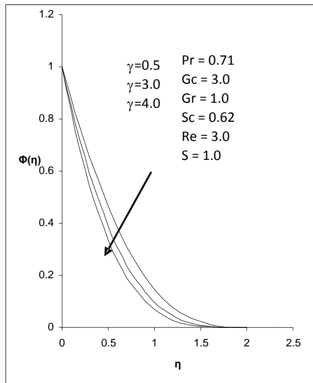
Fig (9) Chemical reaction over the concentration profiles.
