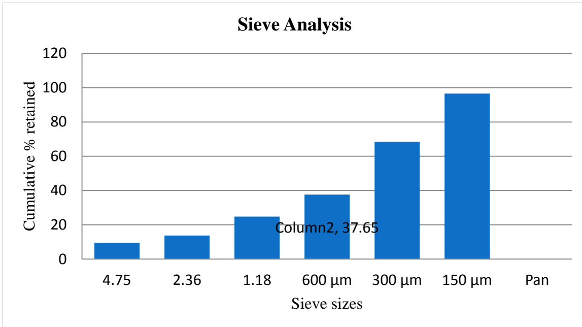
Figure:3.1 Sieve Analysis of Sand
