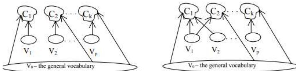
(a) Concepts of queen. (b) Complicated concepts
