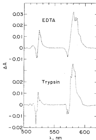
Fig. 1. Absorption spectra of neodymium (III) at pH 5.6 with EDTA and trypsin. reconstruction based on Darnall et al. Concentrations: EDTA 87.5 mM, Nd 3+ 26 mM, trypsin 0.37 mM, Nd 3+ 3.74 mM.
